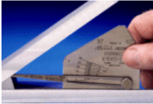
Checking Weld Acute Side
