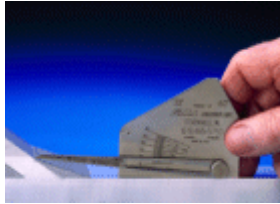
Checking Weld Obtuse Side
