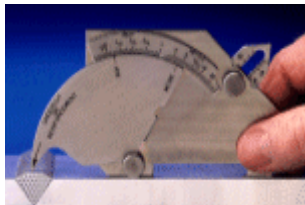
Excess Weld Metal
